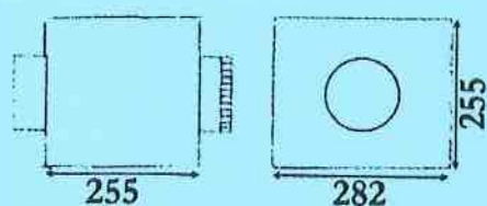
Dimensions (mm) Ecran Box
